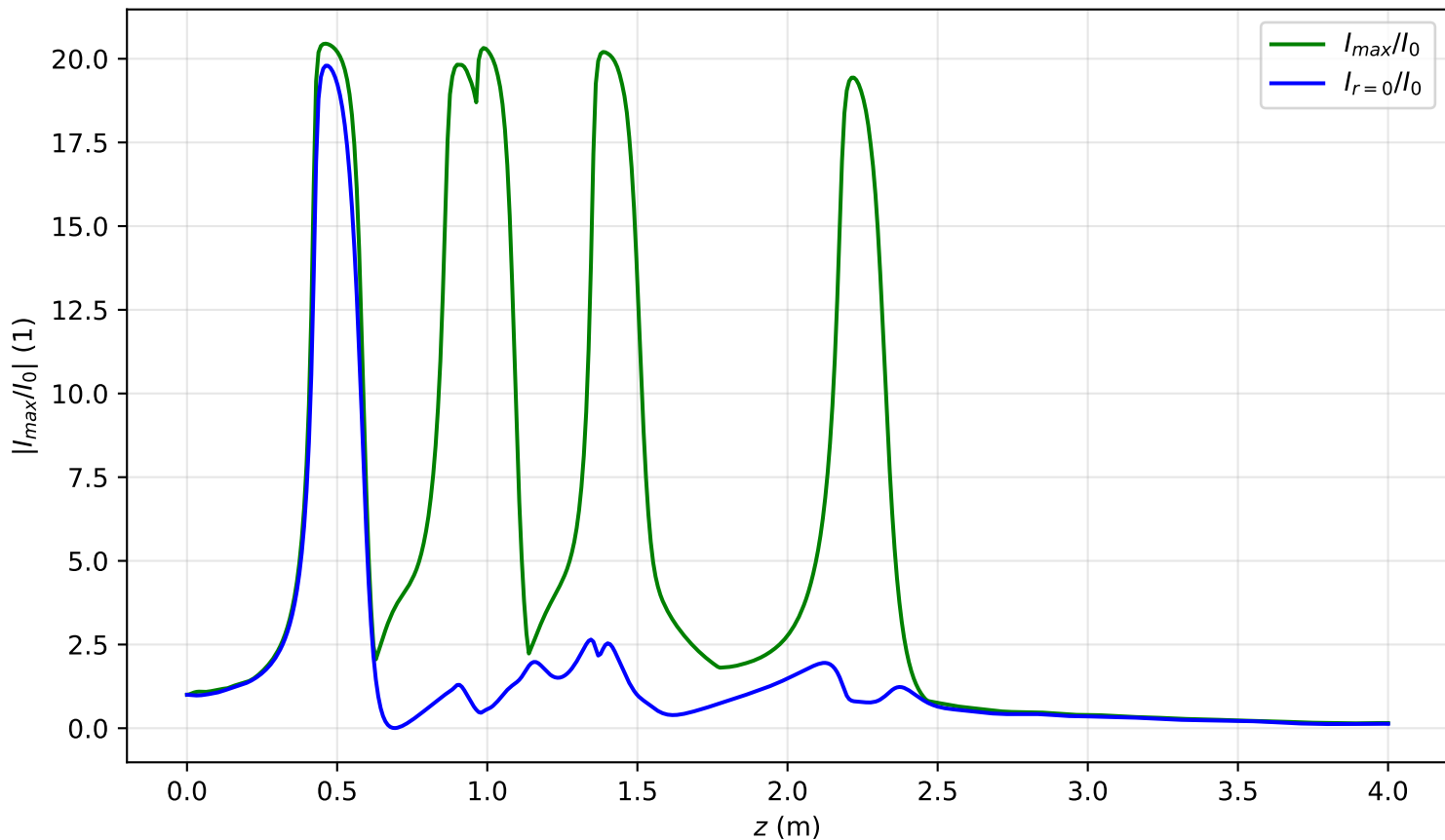
I_{max}(x = 0, y = 0, z)/I_0 , P_{in}=5.4P_{cr} , noisy input, artificial time
